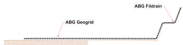
Fig. 5b: Drainage geocomposite Fildrain placed under geogrid
