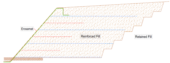
Fig. 8: Completed slope, trimmed face with Erosamat fitted.
