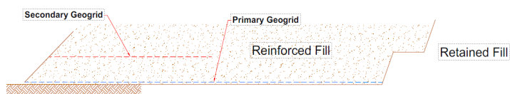
Fig. 6: Primary and Secondary geogrids
