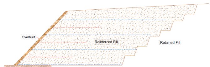
Fig. 7: Design height is built, additional fill build up at the face to be trimmed.
