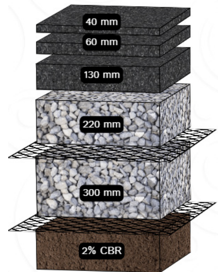
Designed Pavement Section
