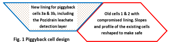
Fig. 1 Piggyback cell design
