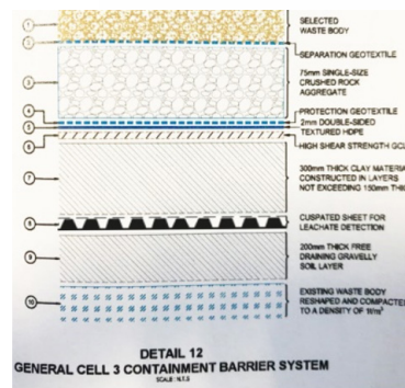
Fig. 4 Lining, leachate management and drainage layers for existing cell remediation and new piggyback cells
