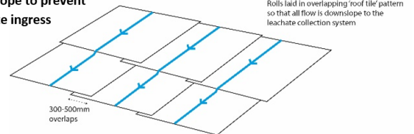
Fig. 4 Lining, leachate management and drainage layers for existing cell remediation and new piggyback cells
