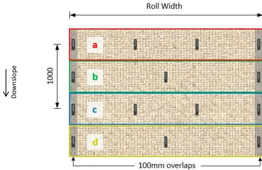
Pinning Pattern PB-3
