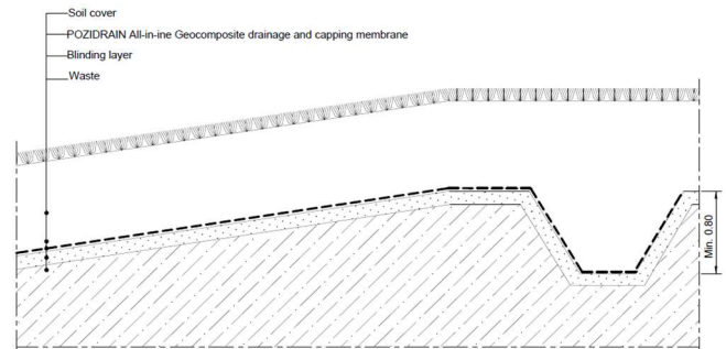
Fig. 12: Pozidrain laid in anchor trench
