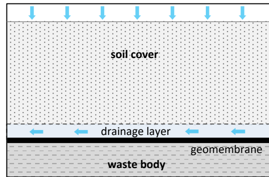
Figure 1: Typical Landfill Capping
