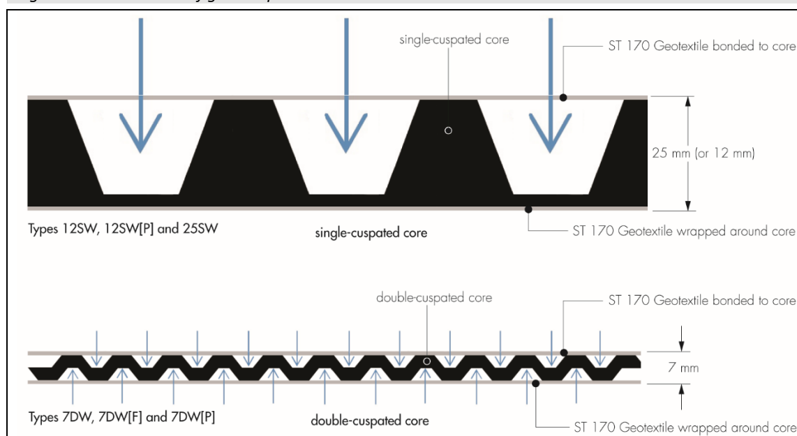
Figure 1 Cross section of geocomposite
