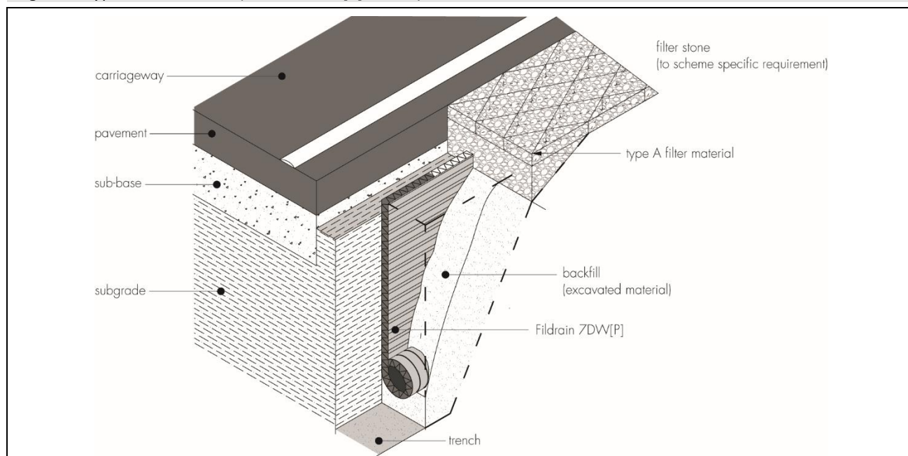
Figure 2 Typical installations (Fildrain 7DW[P] shown)
