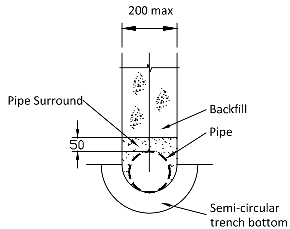
ALTERNATIVE TRENCH SHAPE For drain types 6 and 7
