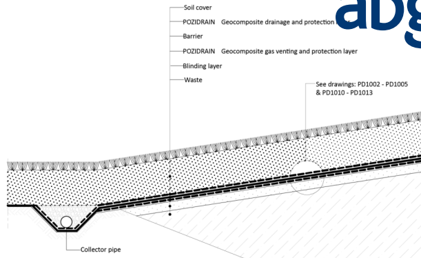
Fig. 12: Collector pipe outfall trench
