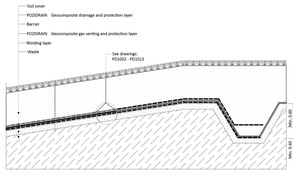
Fig. 12: Pozidrain laid in anchor trench
