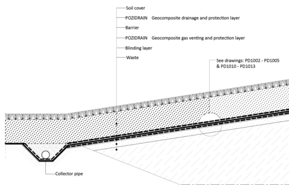
Fig. 13: Collector pipe outfall trench
