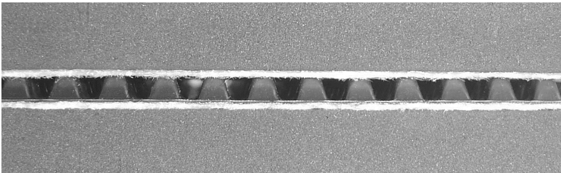
Figure 3 - Soft platen test and cuspatated geocomposite drainage sheets at 35kPa pressure.
