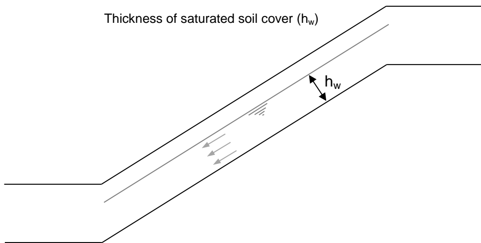
Figure 5 - Insufficient drainage capacity resulting in water flow within the soil cover along the slope
